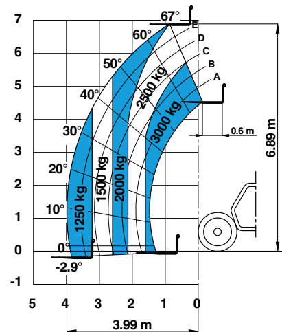
Lift capacity chart
